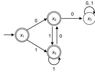
Fig. 4 Finite state machine produced by merging 1-equivalent states x_2 and x_4
